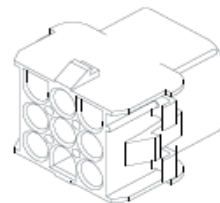
9 Position Connector (Female) # E307428 Terminals (Female) # E307147
