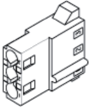
3 Position Connector (Male) # E502101 Terminals (Female) # E307379
