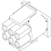
6 Position Connector (Male) # E502104 Terminals (Male) # E307112
