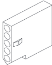
5 Position Connector (Male) # E305005 Terminals (Male) # E307117
