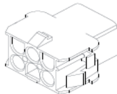
6 Position Connector (Female) # E307375 Terminals (Female) # E307147
