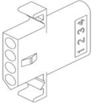
4 Position Connector (Male) # E307077 Terminals (Female) # E307117
